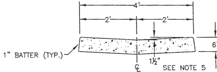
P.C.C. VALLEY GUTTER DETAIL
