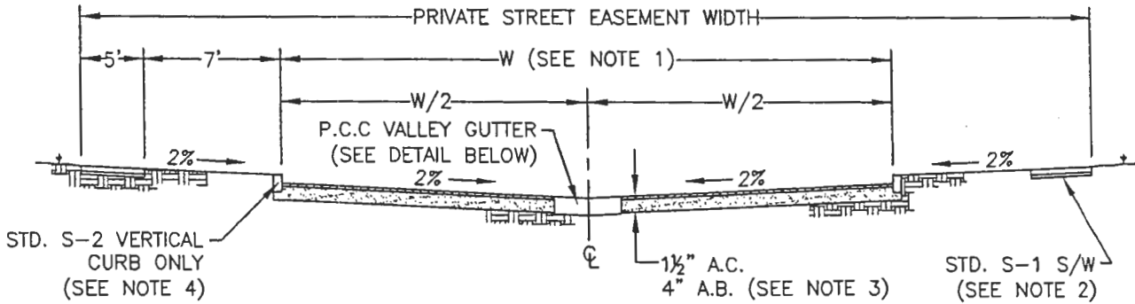
VALLEY GUTTER SECTION
