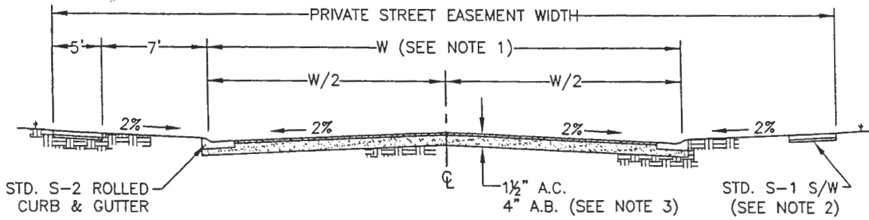
CROWNED SECTION
