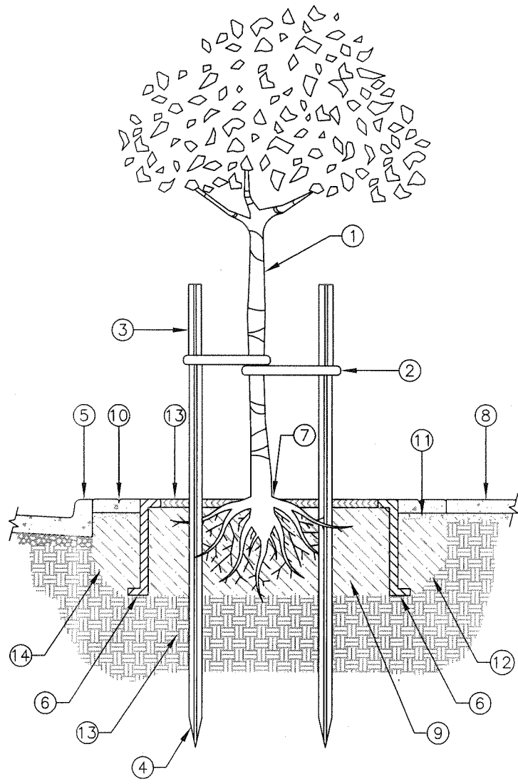
SECTION VIEW
