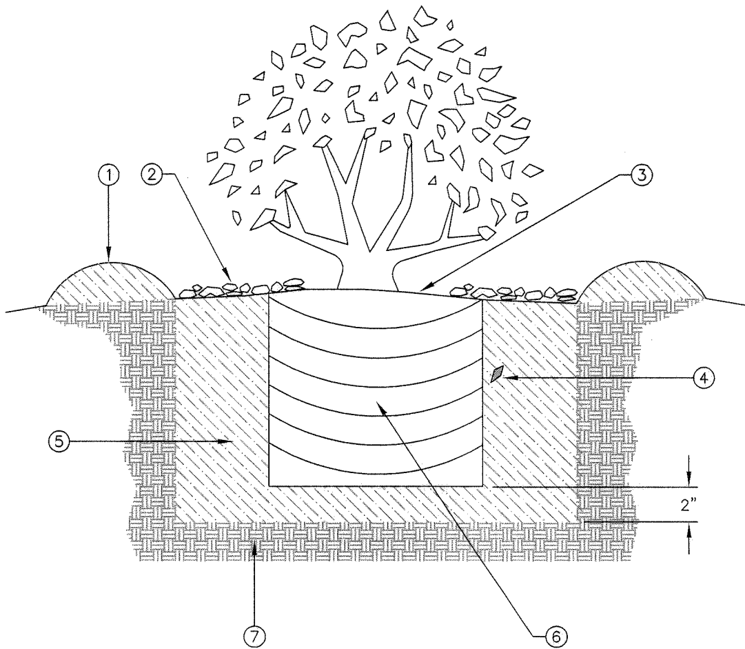
SECTION VIEW
