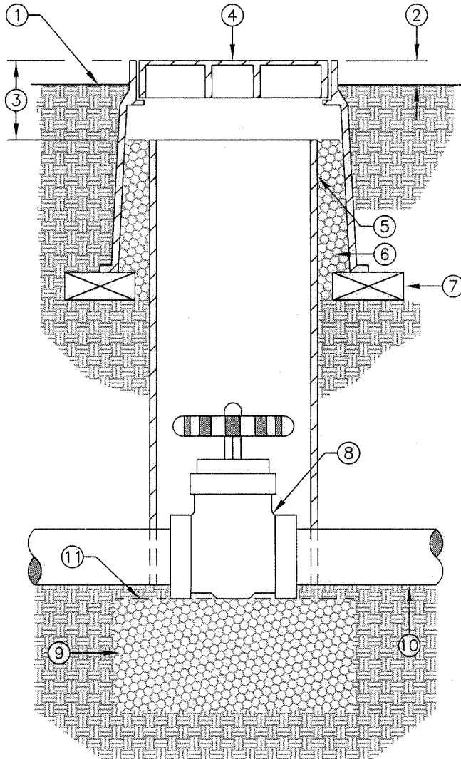
SECTION VIEW
