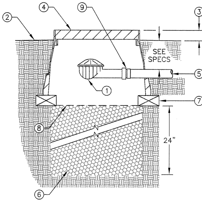
SECTION VIEW
