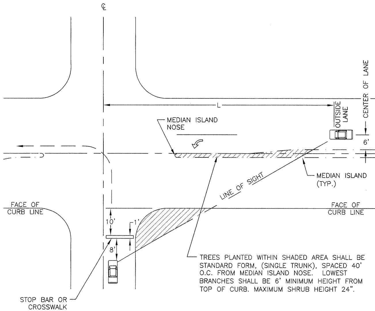
PLAN VIEW
