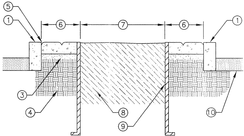
SECTION VIEW AT TREE
