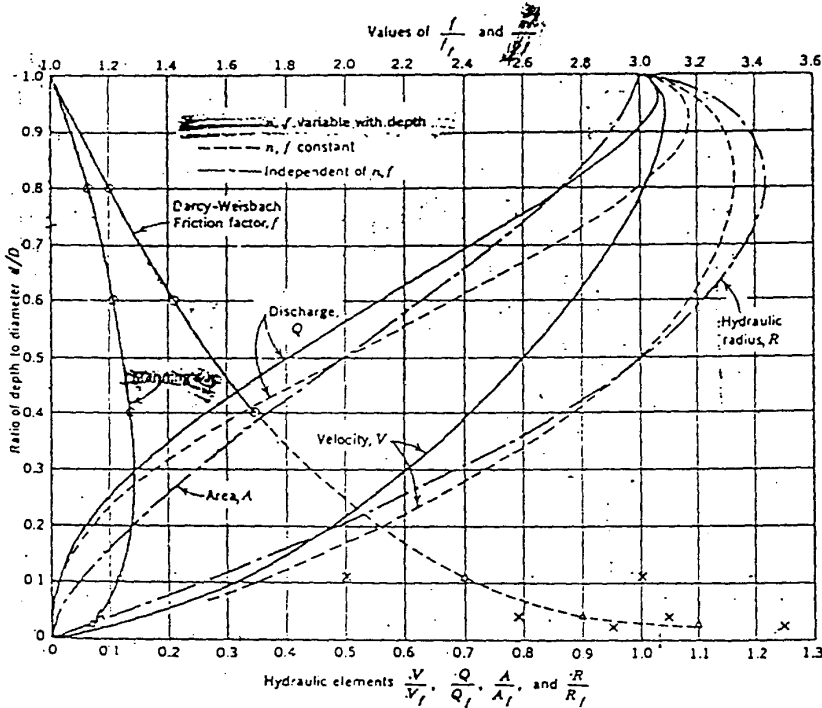
FIGURE 24.—Hydraulic-elements graph for circular sewers.
