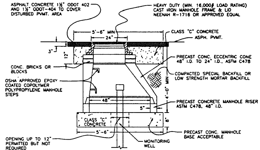
SECTIONAL VIEW UNDER ASPHALT PAVEMENT
