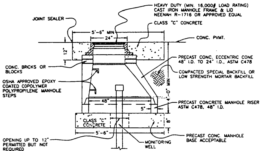
SECTIONAL VIEW UNDER CONCRETE PAVEMENT
