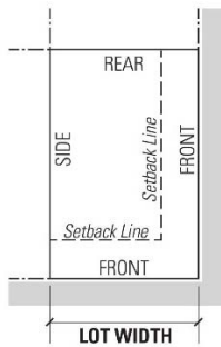
LOT WIDTH Corner Lot
