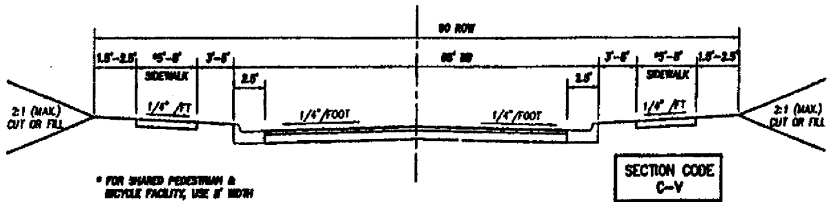
Major Thoroughfare – Five Lane
