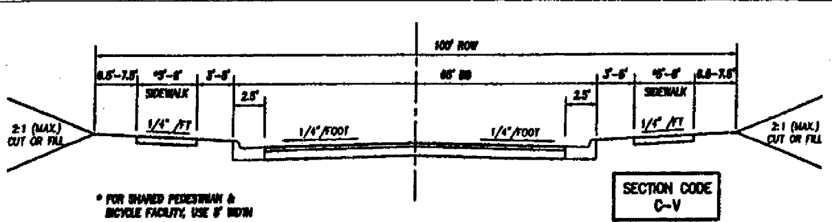
Major Thoroughfare – Five Lane
