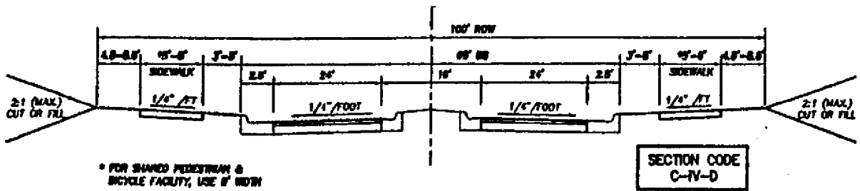
Major Thoroughfare – Four Lane Divided
