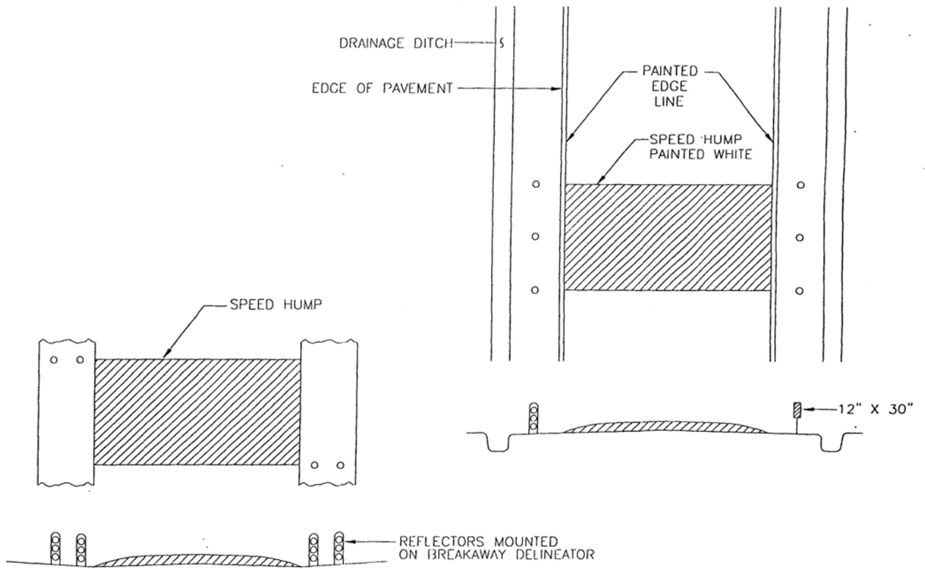
VALENCIA COUNTY FIGURE 3 ALTERNATIVE SPEED HUMP DESIGN FOR STREET W/O C&G
