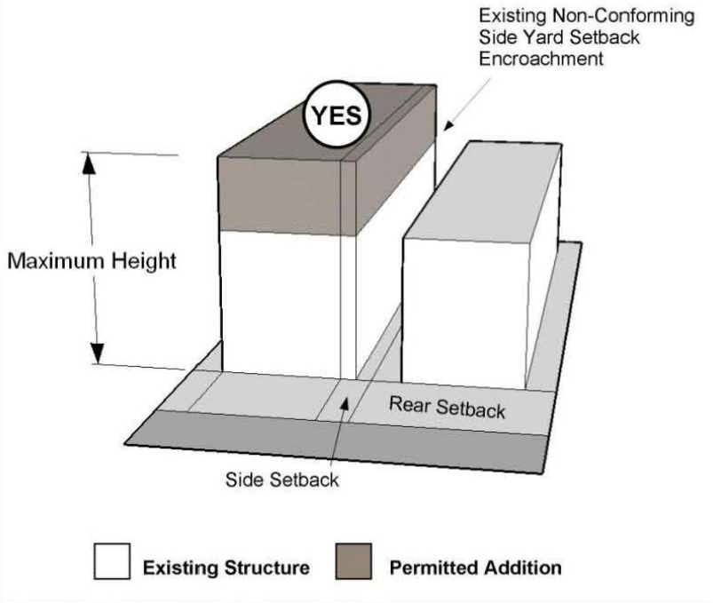
Vertical Extension of Non-conforming Side Wall
