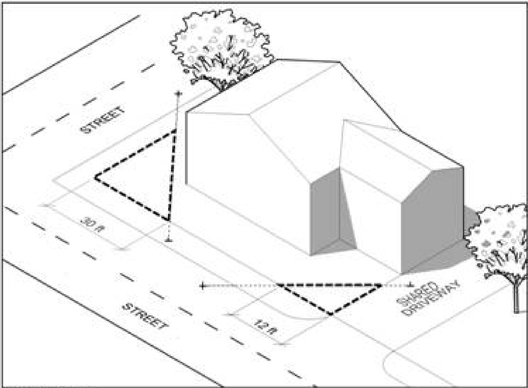
Sight triangles
